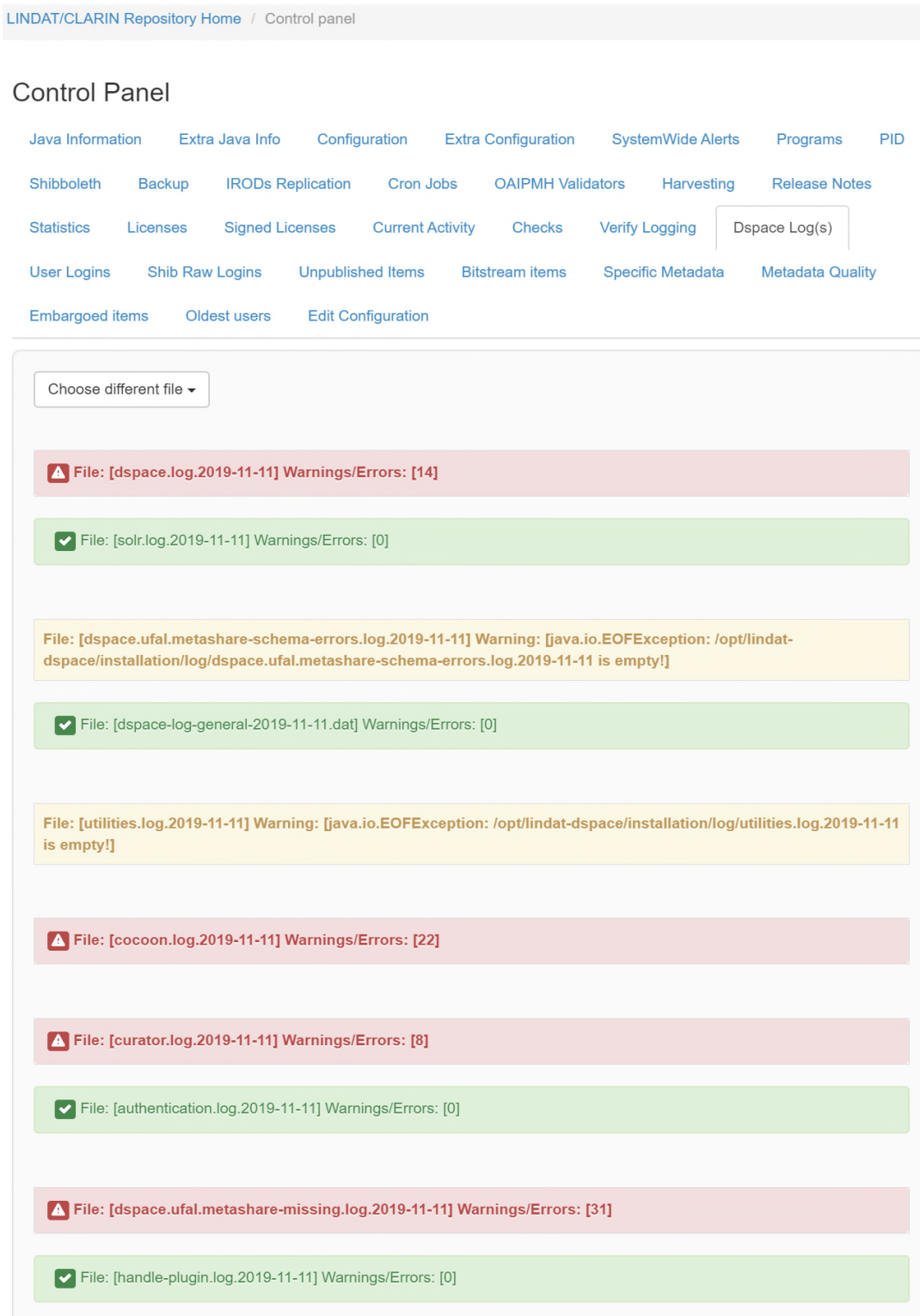
Figure 1: An illustration of control panel with logs tab selected. This provides a brief overview of various log files of the system and allows to inspect them without using the command line.
